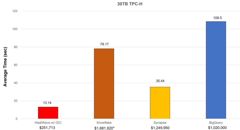
FIGURE 5: HEATWAVE TPC-H PERFORMANCE
