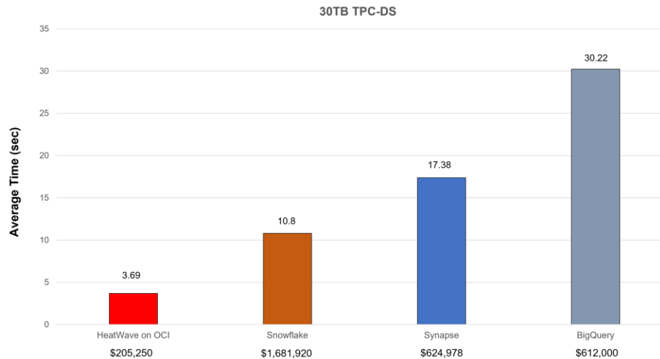
FIGURE 6: HEATWAVE TPC-DS PERFORMANCE
